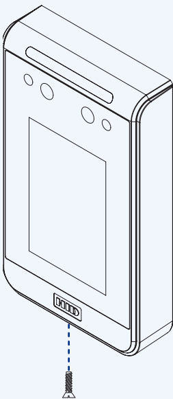
4. Secure the reader to the mounting plate using the supplied screw.
