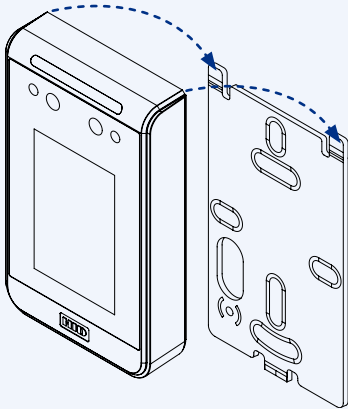
2. Insert the reader into the mounting plate.
